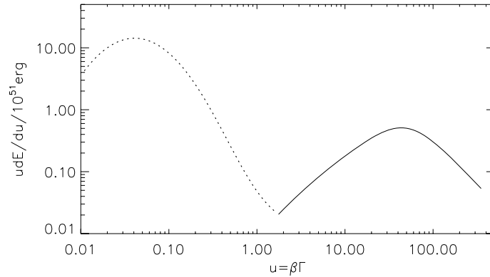
Figure 1. Schematic figure showing dE/d\ln u , in units of 10^{51} erg, as a function of u \equiv \Gamma\beta = (\Gamma^2 - 1)^{1/2} . It has one relativistic component (solid line) with total energy \sim 10^{51} erg and a peak at u \sim 30\text{--}50 that produces the GRB and the afterglow radiations. The power-law index above the peak for this component is well constrained by the X-ray data (the shallow part of the light curve) and is \sim -1.5 (see Table 1). The slope below the peak is not constrained and is taken to be 1; in reality it can be close to zero, as the only constraint we have is from late-time radio afterglow observations which suggests that there is not a lot of extra energy in material moving with Lorentz factor of the order of 2. The second component (dotted curve) shows schematically the kinetic energy in non-relativistic ejecta in the supernova accompanying the GRB; the peak for this component is taken to be \sim 10^4 km s ^{-1} , the typical velocity for Type Ic supernova ejecta, and the energy is \sim 10^{52} erg.
