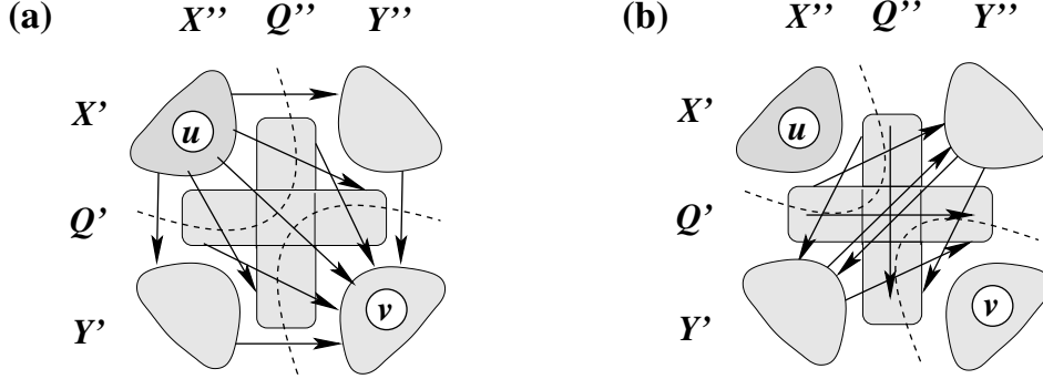
Fig. 2. Illustration to the proof of Proposition 2.8.
