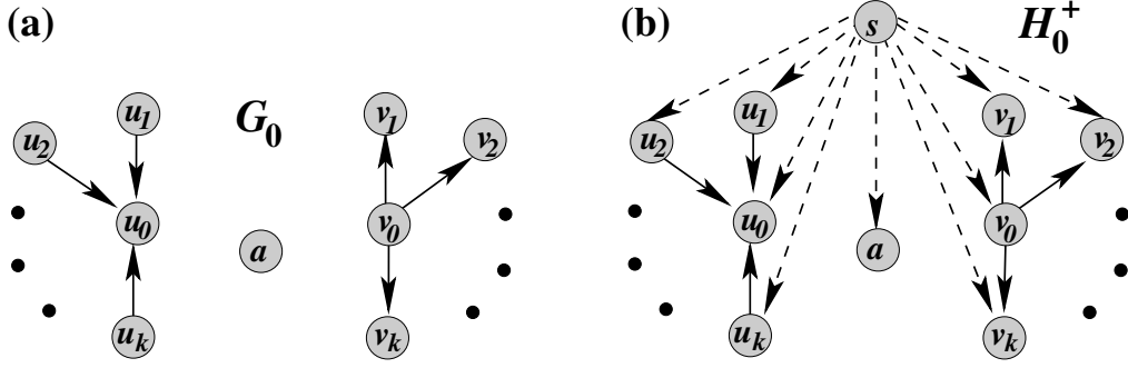
Fig. 1. An example of construction of H_0^+ . (a) An instance G_0, r of CA: the requirements are r(u_i, v_j) = 1 , i, j = 1, \dots, k , and r(u, v) = 0 otherwise. (b) The graph H_0^+ (the requirements remain the same, edges added are shown by dashed lines).
