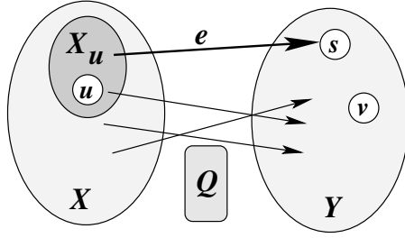
Fig. 3. Illustration to the proof of Corollary 2.9.
