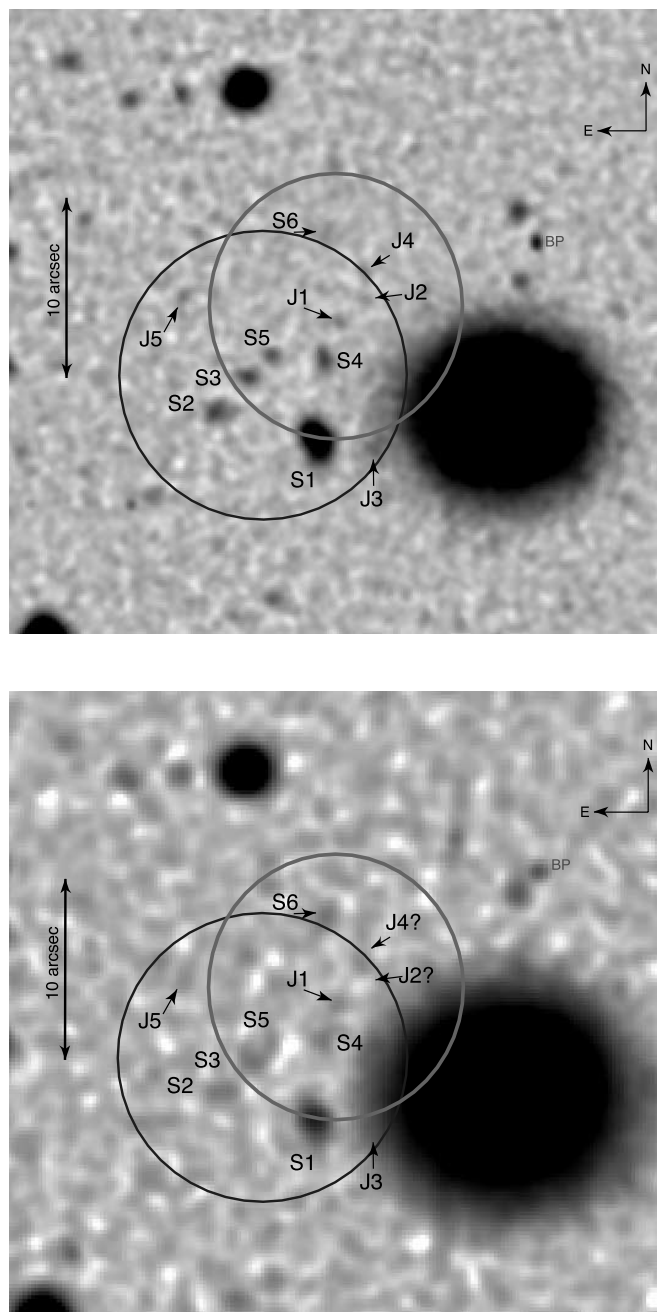
FIG. 1.—Keck LRIS G -band (top) and R -band (bottom) images, zoomed to show the XRT error circle. The larger, lower circle is the revised XRT position from Rol et al. (2005); the smaller, upper circle to the west and north of that is our 2\sigma confidence region (see text) of the XRT position. The images have been median-subtracted and smoothed to accentuate the detection of faint sources under the glare of the bright galaxy G1. The 11 sources consistent with the Rol et al. (2005) X-ray afterglow localization are labeled in both images, with the astrometric positions given in Table 2. North is up and east is to the left. G1 is the large galaxy to the west and south of the XRT. Bad pixel locations are denoted with “BP.” [See the electronic edition of the Journal for a color version of this figure.]
