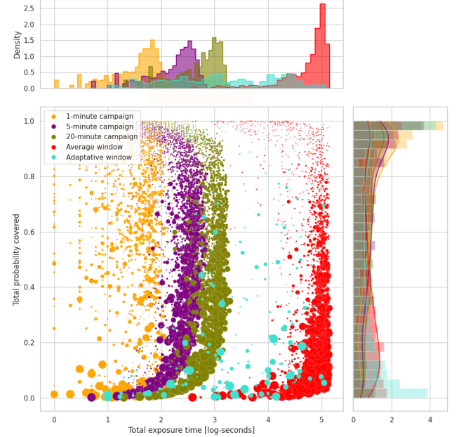
Figure 9. Total GW location uncertainty (named probability for simplicity) covered in terms of the total exposure time for the five configurations explored in this work. The size of the markers corresponds to the size of the GW uncertainty regions, depicted for qualitative considerations.
