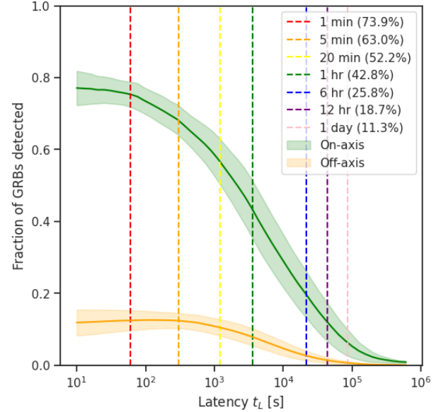
(d) Fraction of on- and off-axis events detected with increasing latency after GRB onset
