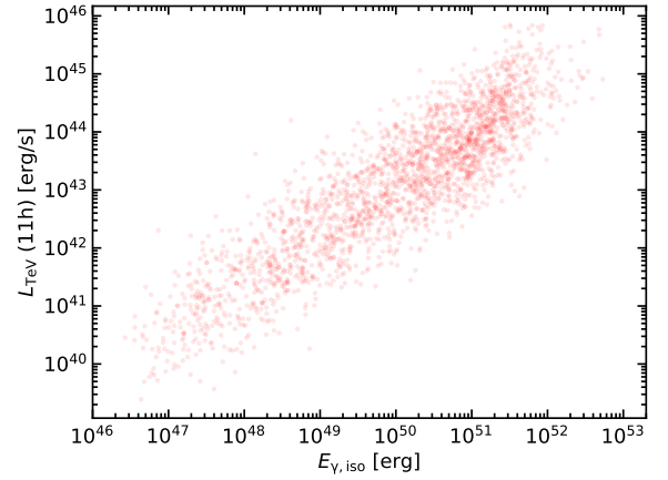
Figure 2. TeV luminosity at 11 hr versus E_{\gamma,\text{iso}} for the sample of short GRBs simulated in this work.
